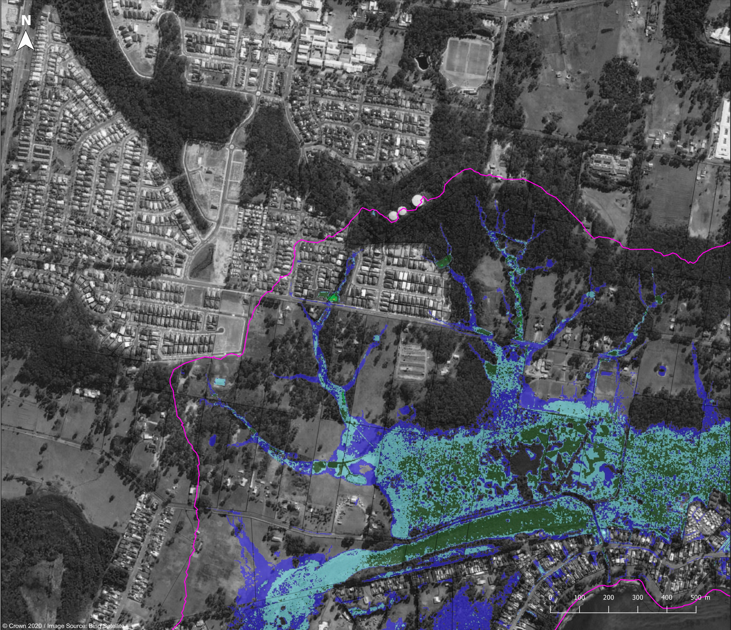
Figure D1.2 1% AEP Flood Life Hazard Categories
